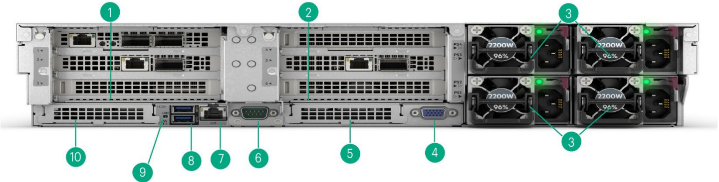
HPE ProLiant Compute DL384 Gen12 – Rear View
