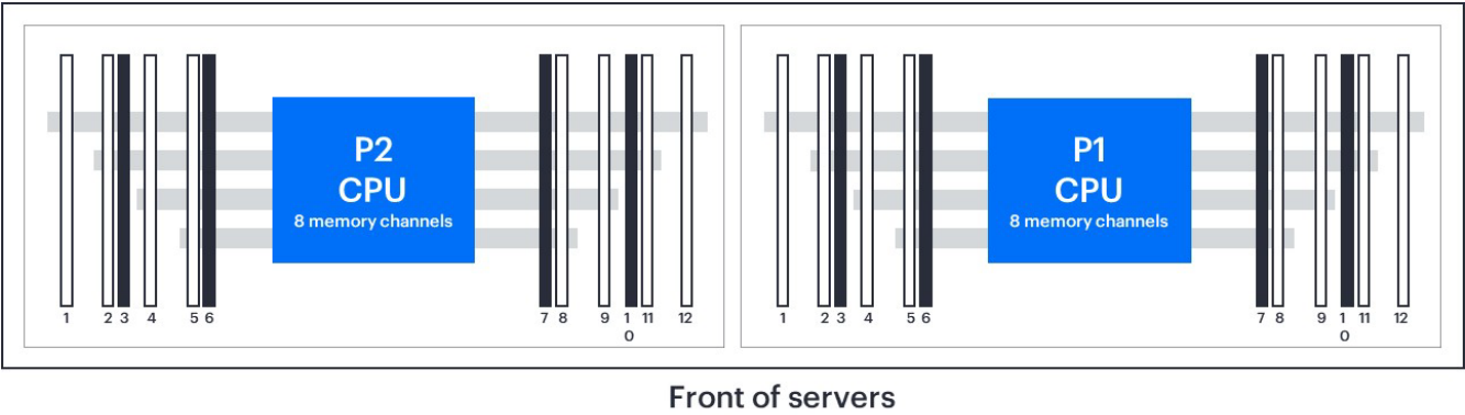
Figure 9. DIMM slot locations in HPE Alletra 4120/4110 and HPE ProLiant DL380a Gen11 servers
