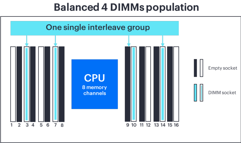
Figure 2. Example of memory that has balanced population
