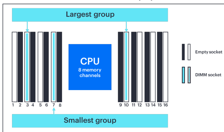
Figure 3. Example of memory that has unbalanced population
