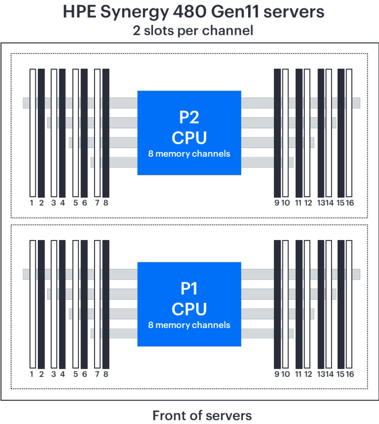
Figure 8. DIMM slot locations for HPE Synergy 480 Gen11 Compute modules (P1 and P2 are rotated)
