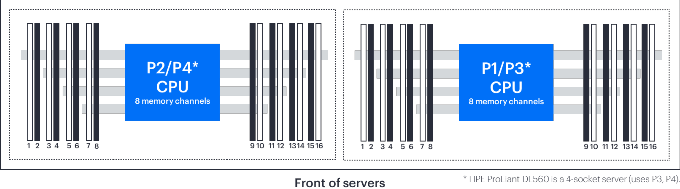
Figure 6. DIMM slot locations in HPE ProLiant DL360/DL380/ML350/DL560 Gen11 servers
