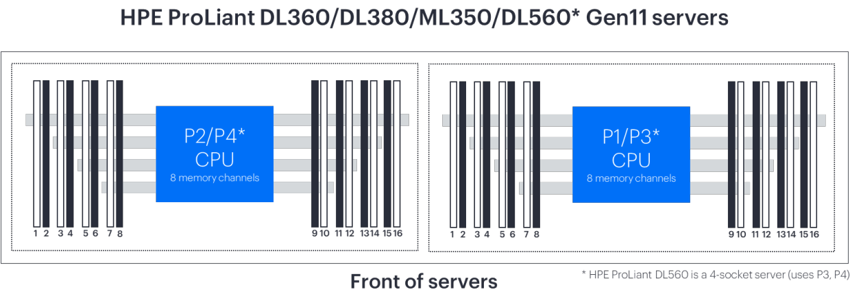
Figure 1. 32 DIMM slot locations in HPE ProLiant DL360/DL380/ML350 and 64 DIMM slot locations in HPE DL560 Gen11 servers
