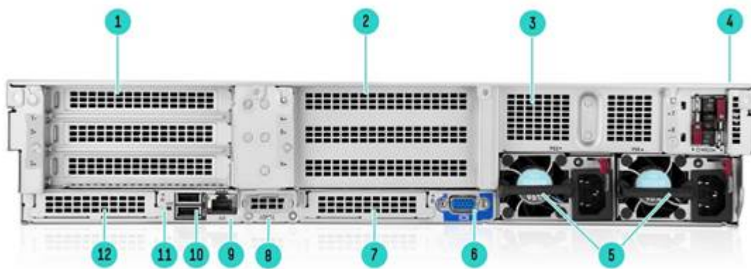
Rear View - DL380 Gen12 Air Cooled
