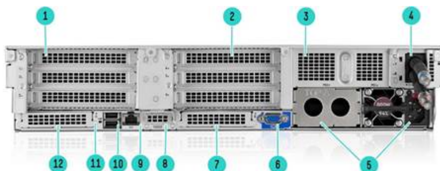
Rear View - DL380 Gen12 Direct Liquid Cooling
