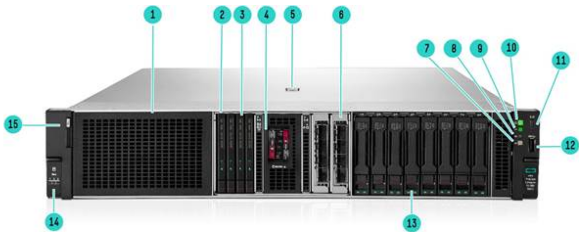
Front View - 8SFF chassis with optional multi-purpose cage
