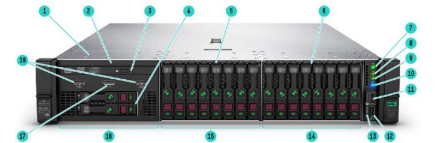
HPE ProLiant DL385 Gen10 Server - Front View
