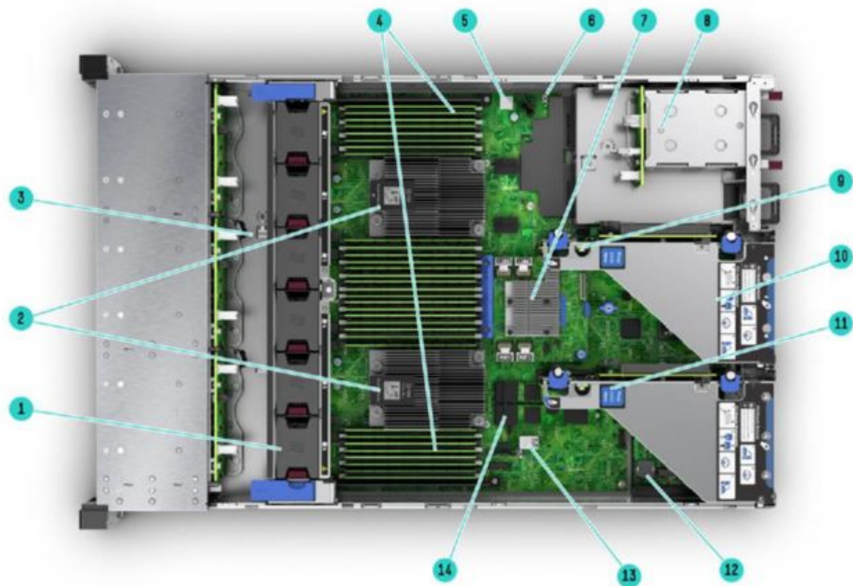
HPE ProLiant DL385 Gen10 Server - Internal View 8SFF chassis with optional 2 nd CPU, FlexLOM, Smart array shown
